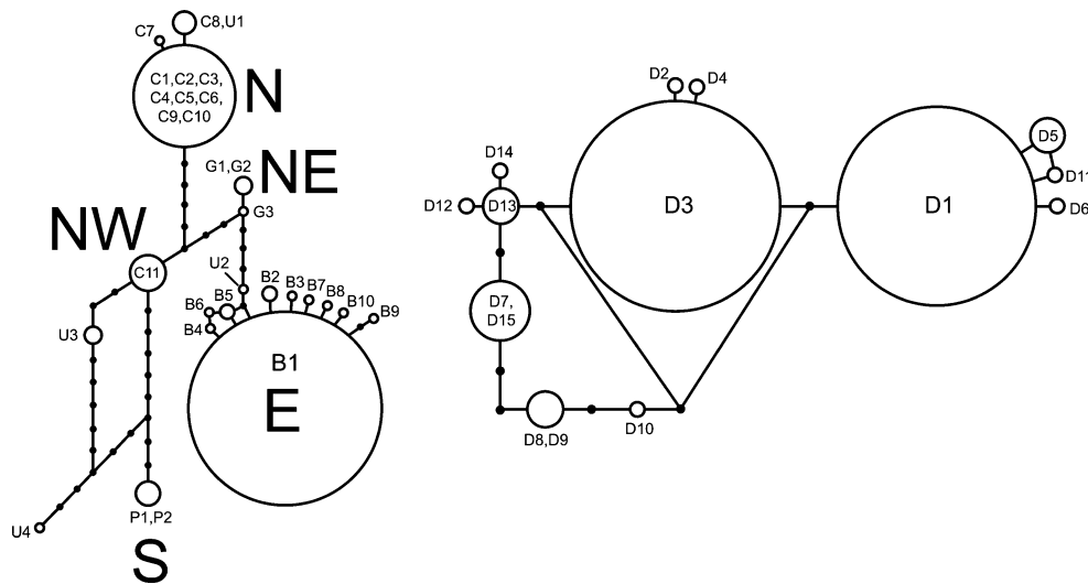
Fig. 3 Parsimony networks for mtDNA haplotypes of Chelonoidis carbonaria (left) and C. denticulata (right), based on alignments of 420 bp. Circle size approximately reflects haplotype frequency. Missing haplotypes are shown as small solid circles. Each line connecting haplotypes corresponds to one mutational step. Large upper-case letters indicate geographic origin of haplotypes within the range of C. carbonaria (N, north; NE, northeast; etc.). Haplotype frequencies for C. carbonaria are B1: n=30 ; (C1, C2, C3, C4, C5, C6, C9, C10): n=16 ; C11: n=6 ; (P1, P2): n=5 ; (C8, U1): n=4 ; (G1, G2):
